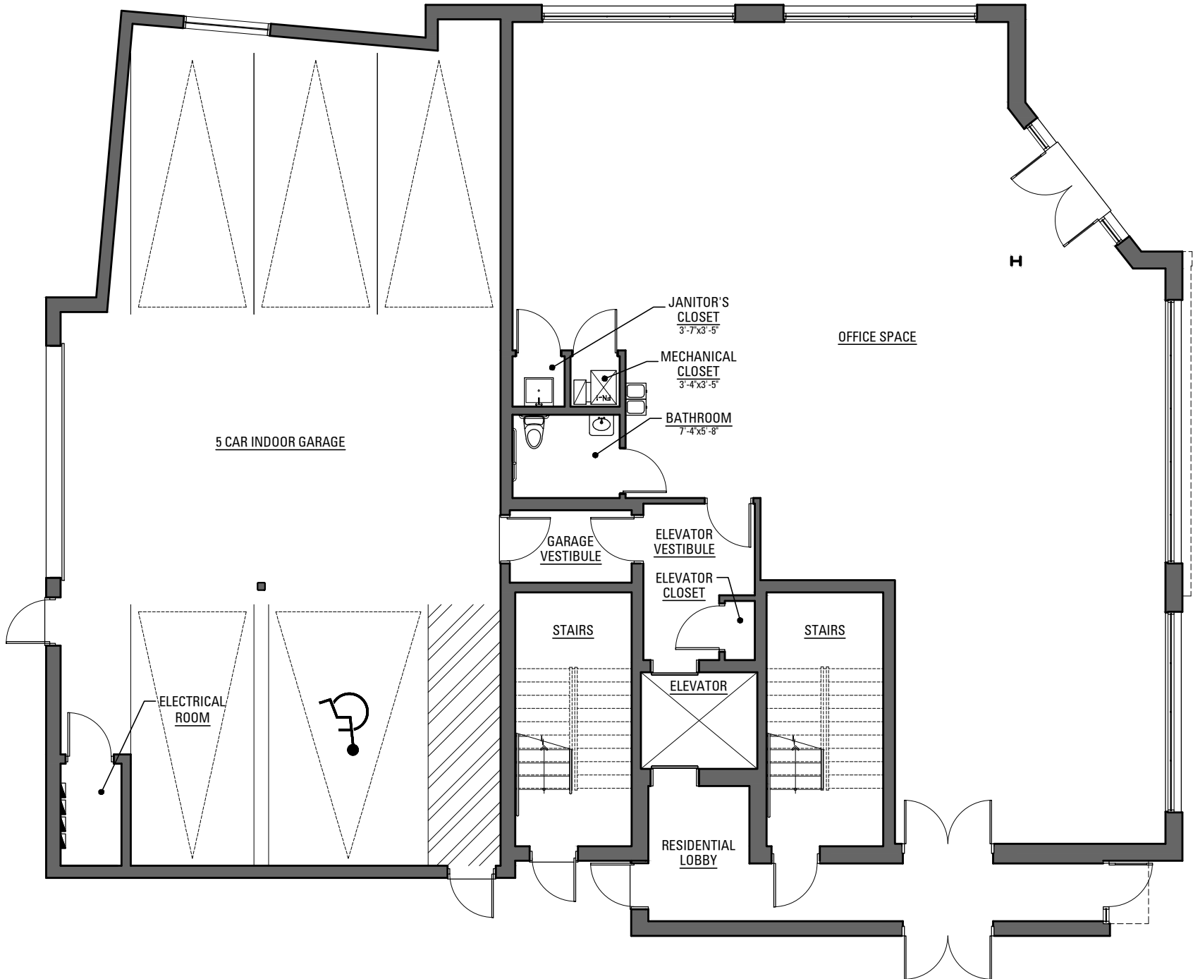
FIRST FLOOR OFFICE SPACE - 2,010 SQ. FT. 2006 W. WEBSTER
